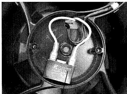
With Capacitor
