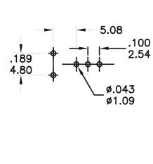
P.C. MOUNTING
