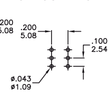
P.C. MOUNTING
