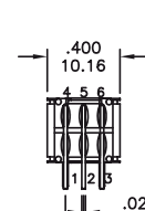
P.C. MOUNTING
