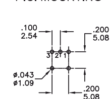
P.C. MOUNTING
